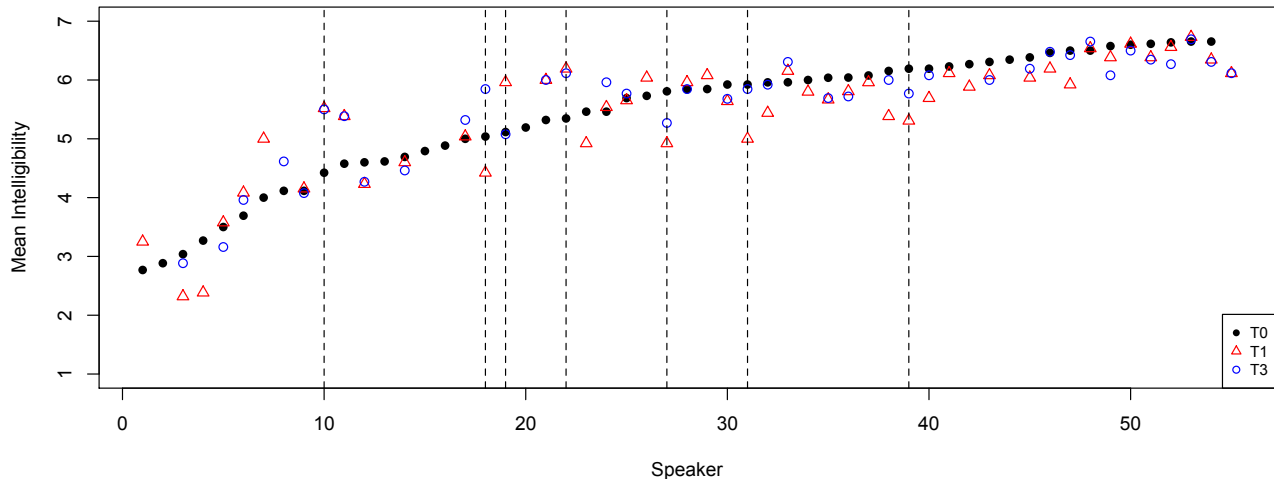
Figure 1: Intelligibility scores for individual speakers at each measurement moment. Data is ordered according to pre-treatment intelligibility score. Dashed lines show the speakers with a significant difference between two or more measurement moments ( p < 0.0013 ). T0 = pre-treatment, T1 = 10-weeks post treatment, T3 = 12-months post treatment.
