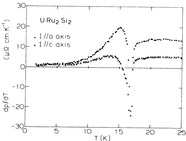
FIG. 3. Temperature dependence of the temperature coefficient d\rho/dT of \text{URu}_2\text{Si}_2 parallel to the a and c axes.
