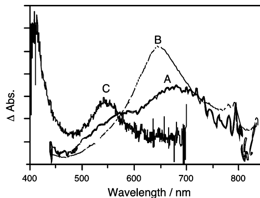
Figure 3. Transient absorption spectra of 1 · 2 and 2 (curves A and B, respectively, 3 ps after flash, in o DCB). The absorption of the free 2^{+} (curve C) was obtained by conventional ns-laser flash photolysis of 2 in the presence of tetracyanoethylene (1:1 CH_3CN/o DCB, \lambda_{\text{ex}} = 355 nm).
