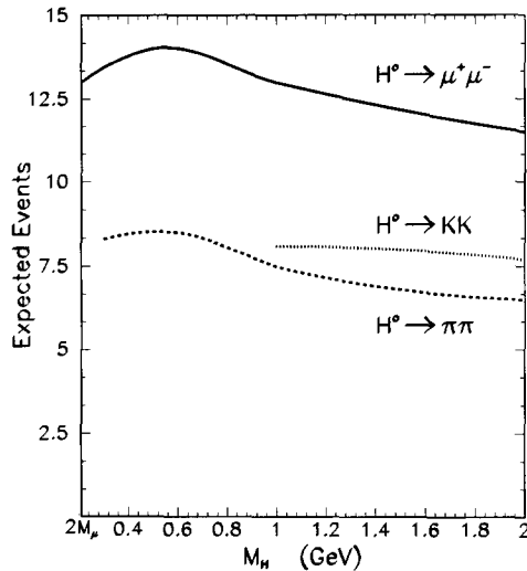
Fig. 2. Number of expected events from the process Z^0 \rightarrow H^0 \ell^+ \ell^- as a function of the Higgs boson mass for three decay channels: H^0 \rightarrow \mu^+ \mu^- , H^0 \rightarrow \pi\pi and H^0 \rightarrow KK .
