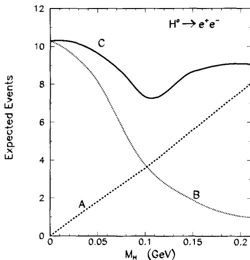
Fig. 3. Number of expected events from process Z^0 \rightarrow H^0 \ell^+ \ell^- as a function of the Higgs boson mass in the range M_{H^0} < 2M_\mu . Curve A is for the case of detected Higgs decay products; curve B is for the search of an Higgs decaying outside the volume of the electromagnetic calorimeter; curve C is the sum of A and B.
