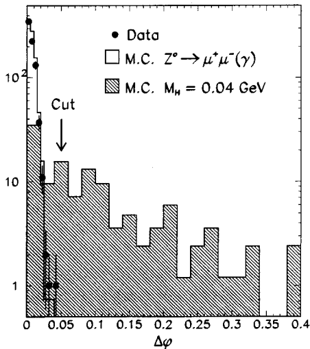
Fig. 1. Acoplanarity angle ( \Delta\phi ) distribution for: Z^0 \rightarrow \mu^+\mu^- data (full points); Z^0 \rightarrow \mu^+\mu^-(\gamma) Monte Carlo (hollow histogram) normalized to the luminosity; Z^0 \rightarrow H^0\mu^+\mu^- Monte Carlo for M_{H^0} = 0.04 GeV (hatched histogram) normalized to twenty times the luminosity. The arrow indicates the \Delta\phi > 0.05 cut described in the text.
