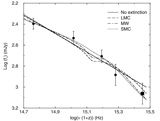
FIG. 6.— BRIJK_s -band spectral energy distribution of the afterglow on 2003 January 26.20 UT. The filled circles represent the RJK_s -band measurements. The filled square is the fiducial B -band photometric point obtained by extrapolating the R -band point using the intrinsic spectral slope ( \beta = 1.32 \pm 0.25 ) derived from the VLT spectrum. The fluxes have been corrected for Galactic extinction (Schlegel et al. 1998). The frequencies are given in the rest frame for z = 3.198 .
