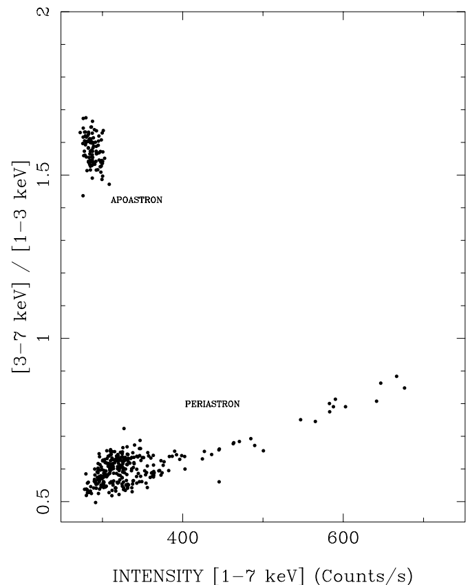
FIG. 1.—Hardness-intensity diagram of Cir X-1. We show in the same box the data at the periastron binary phase (Iaria et al. 2001a) and the new data taken near the apoastron phase, as indicated in the figure. The hardness is defined by the ratio [3-7 \text{ keV}]/[1-3 \text{ keV}] and the intensity of the source is calculated in the energy band [1-7 \text{ keV}] . The bin time is 137 s. The data at the apoastron correspond to lower intensity and higher hardness (top left in the diagram).
