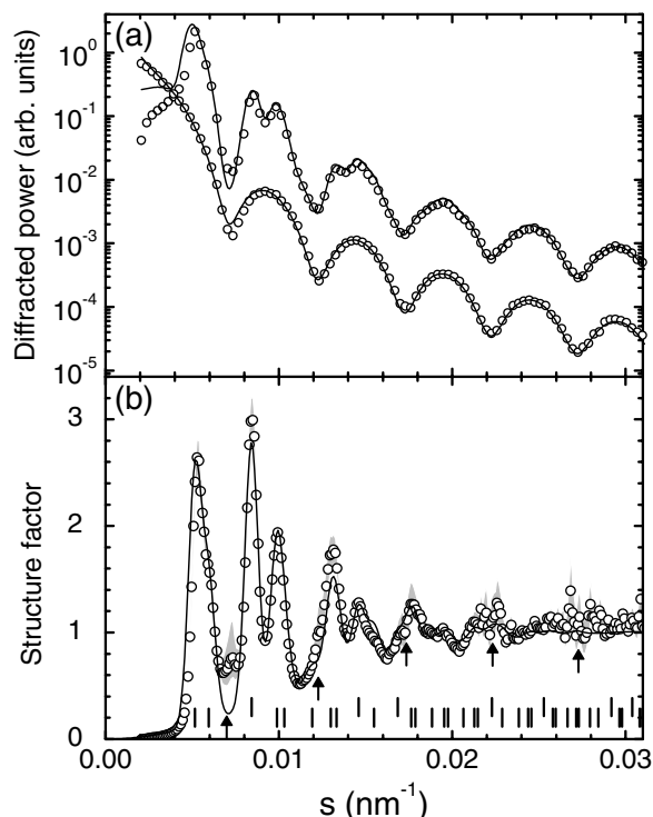
FIG. 1. (a) X-ray diffraction patterns from 100.8 nm radius polystyrene colloidal spheres in methanol, at low density ( <1 vol %, lower curve, form factor) and crystallized (45 vol %, no added resin, upper curve). (b) Structure factor ( \circ ), obtained from the data in (a), together with a model curve for fcc crystals with displacements u = 19.4 \pm 0.5 nm, lattice parameter a = 335.5 \pm 0.7 nm, and 8.7 \pm 1.0\% preferred orientation [26] (—, both panels). The shaded area indicates the experimental accuracy, estimated from Poisson counting statistics and the agreement between measured and calculated data, that was used in the fit. The arrows indicate the minima in the form factor, where the structure factor is less reliable. The marks for reflections from crystals aligned to the cell walls are shifted up.
