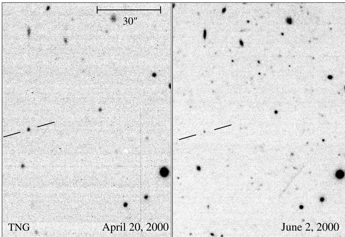
FIG. 1.—Finding chart for the field of GRB 000418. The afterglow is indicated. Left panel : R-band image taken with the TNG telescope on April 20.9 UT. Right panel : R-band image taken with TNG on June 2.9 UT (Table 1). North is up, east is left.
